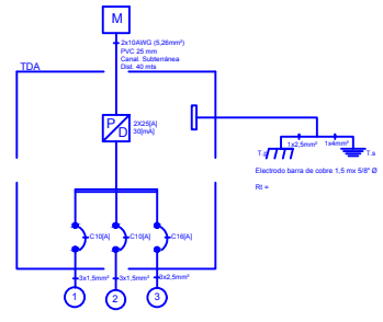
Diagrama Unilineal
